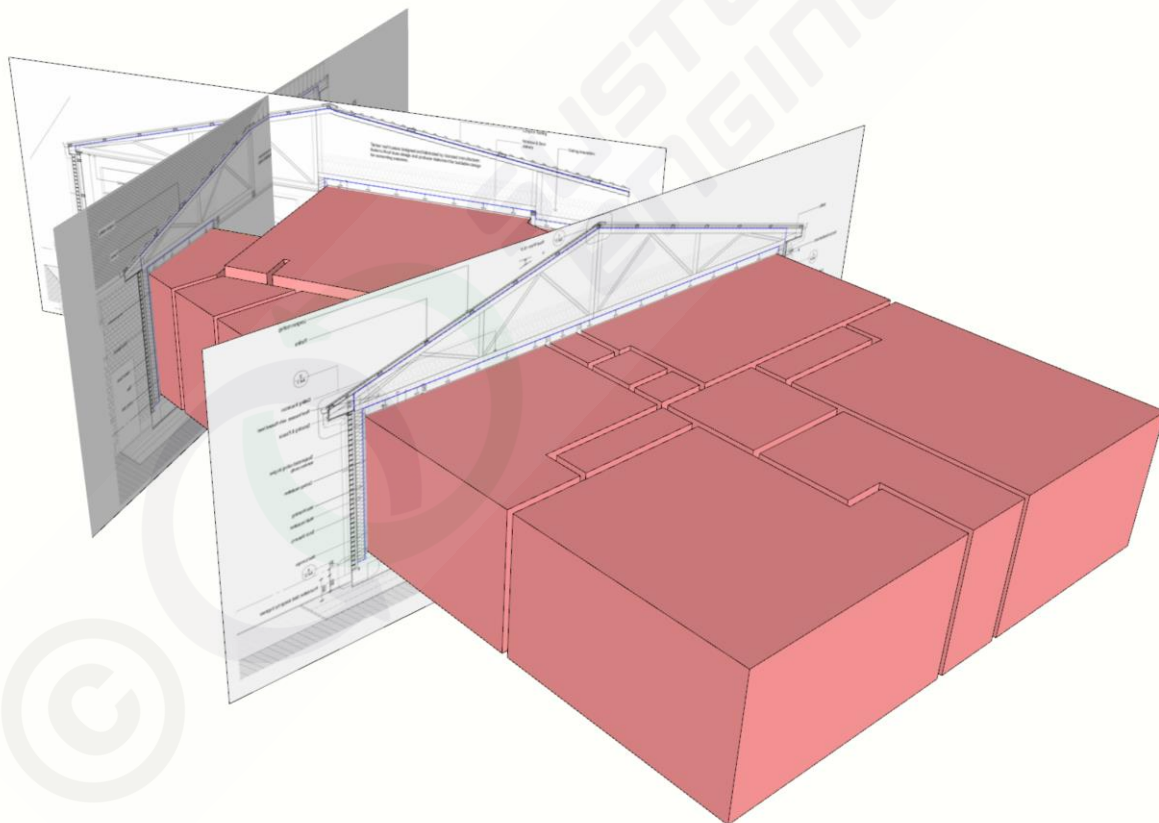
Figure 6: Volume (sections on a different layer)
