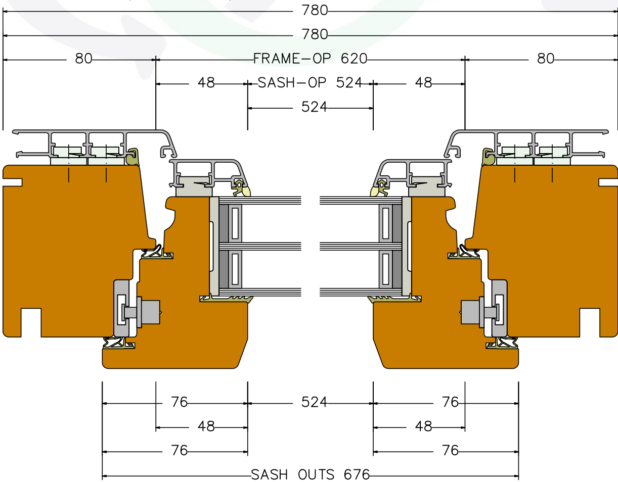
Section H1 (scale 1:2)
