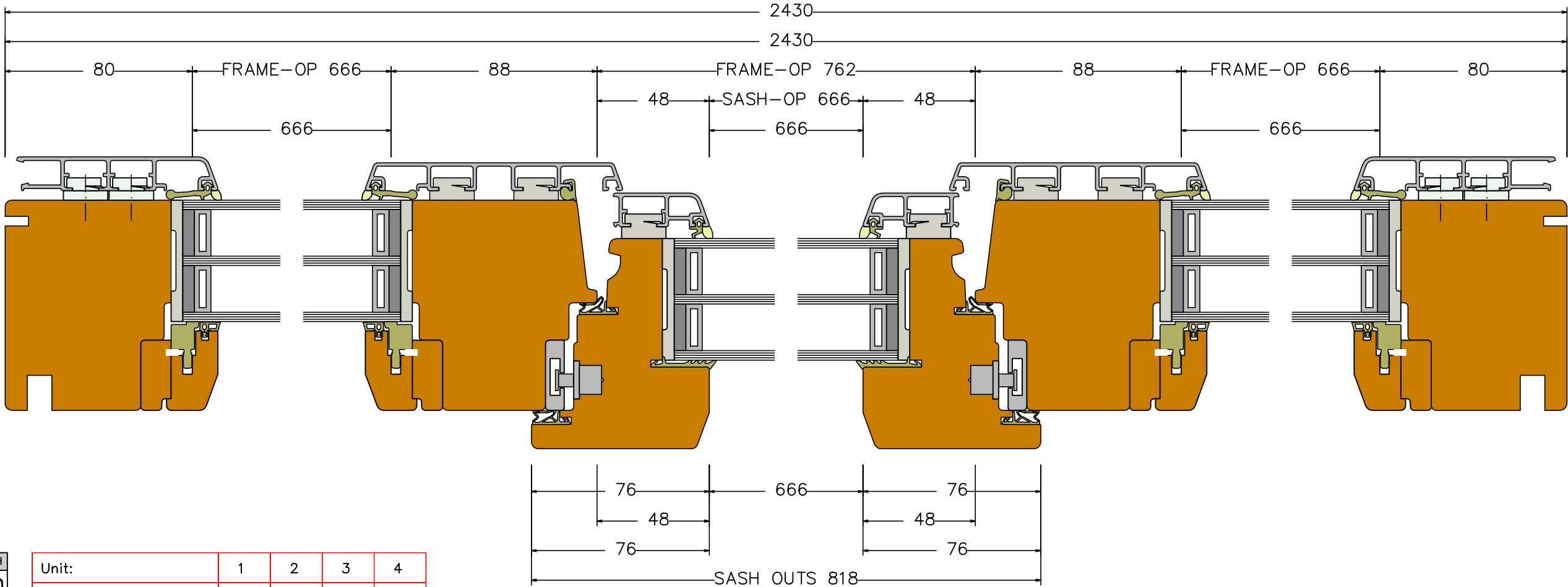
Section H1 (scale 1:2)
