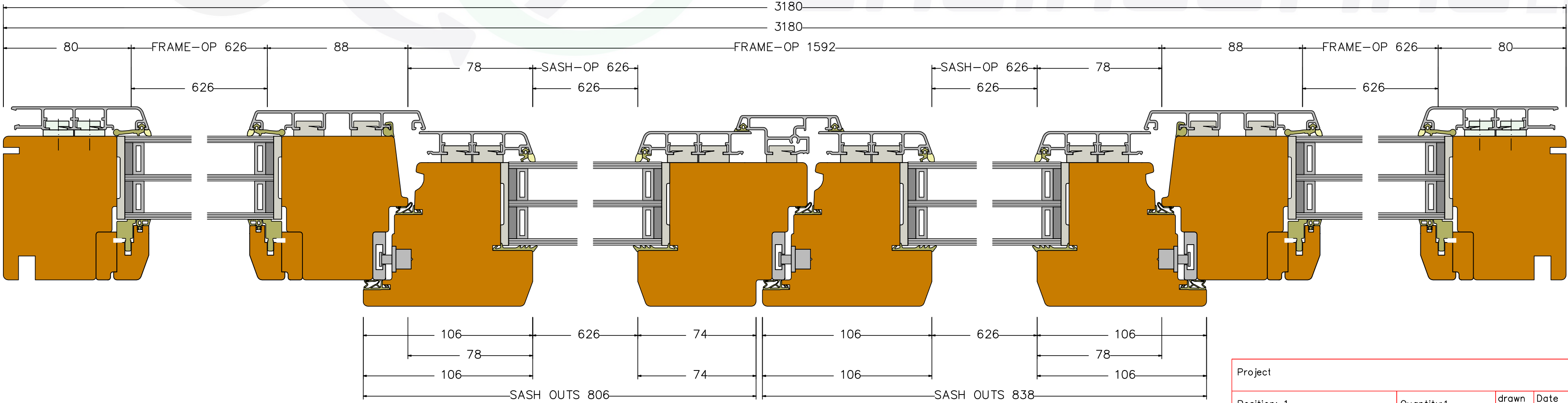
Section H1 (scale 1:2)
