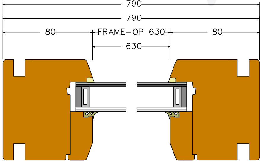
Section H1 (scale 1:2)
