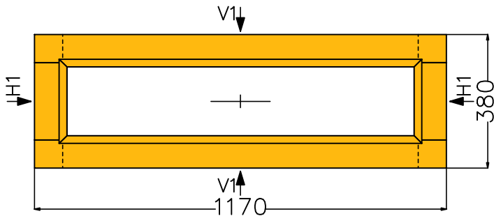
View from inside (scale 1:15)
