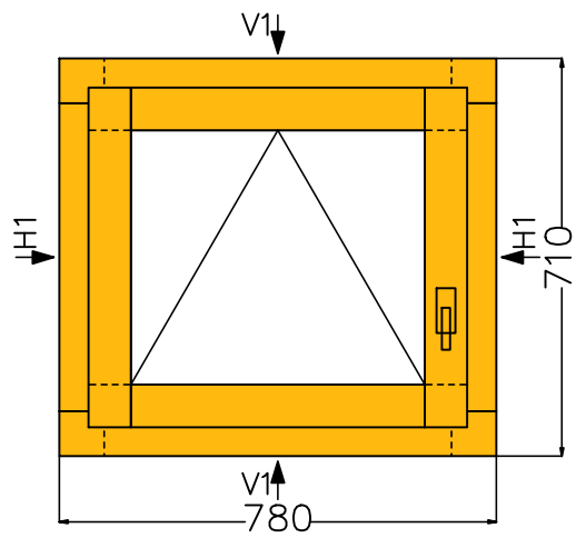
View from inside (scale 1:15)
