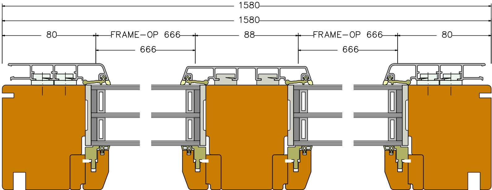
Section H1 (scale 1:2)
