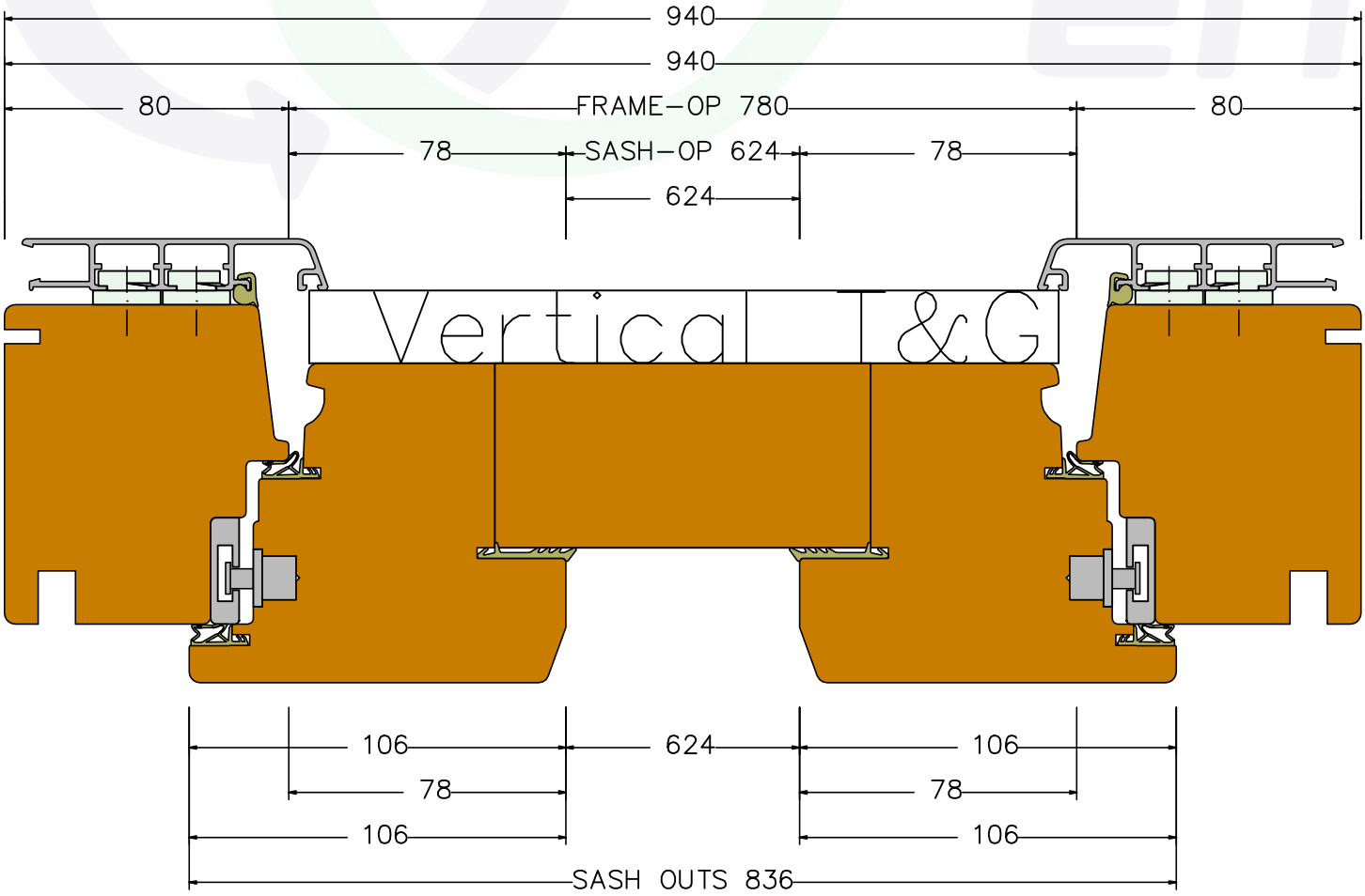
Section H1 (scale 1:2)
