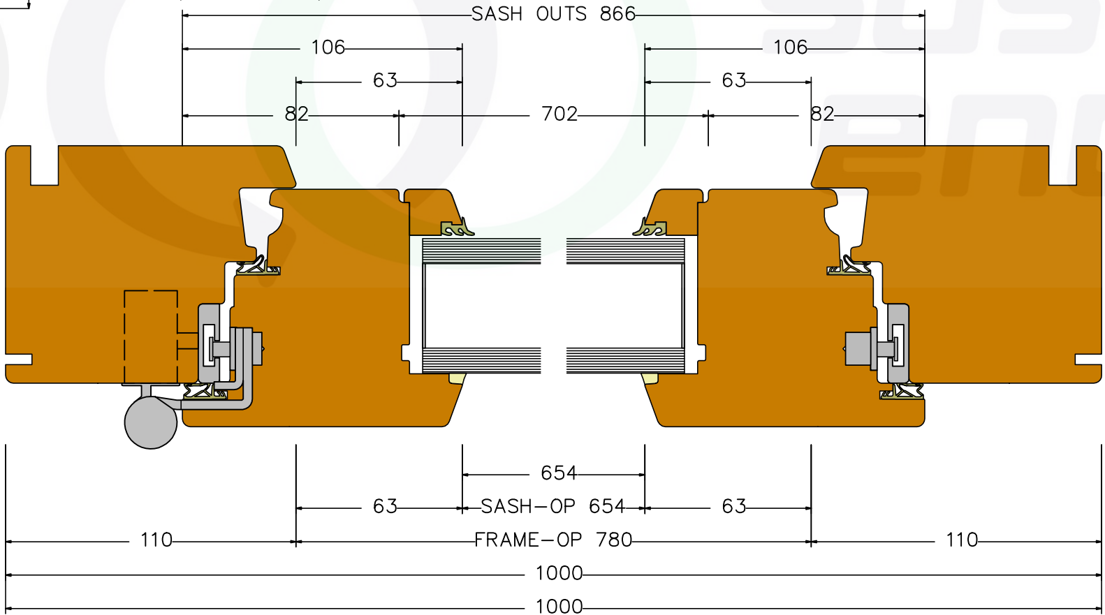
Section H1 (scale 1:2)
