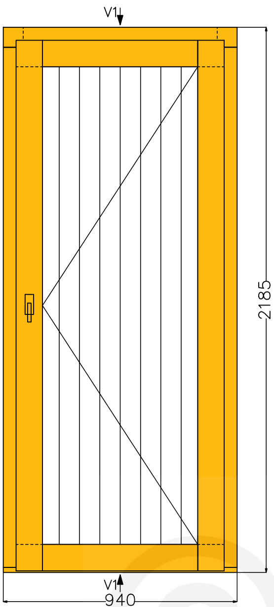
View from inside (scale 1:15)
