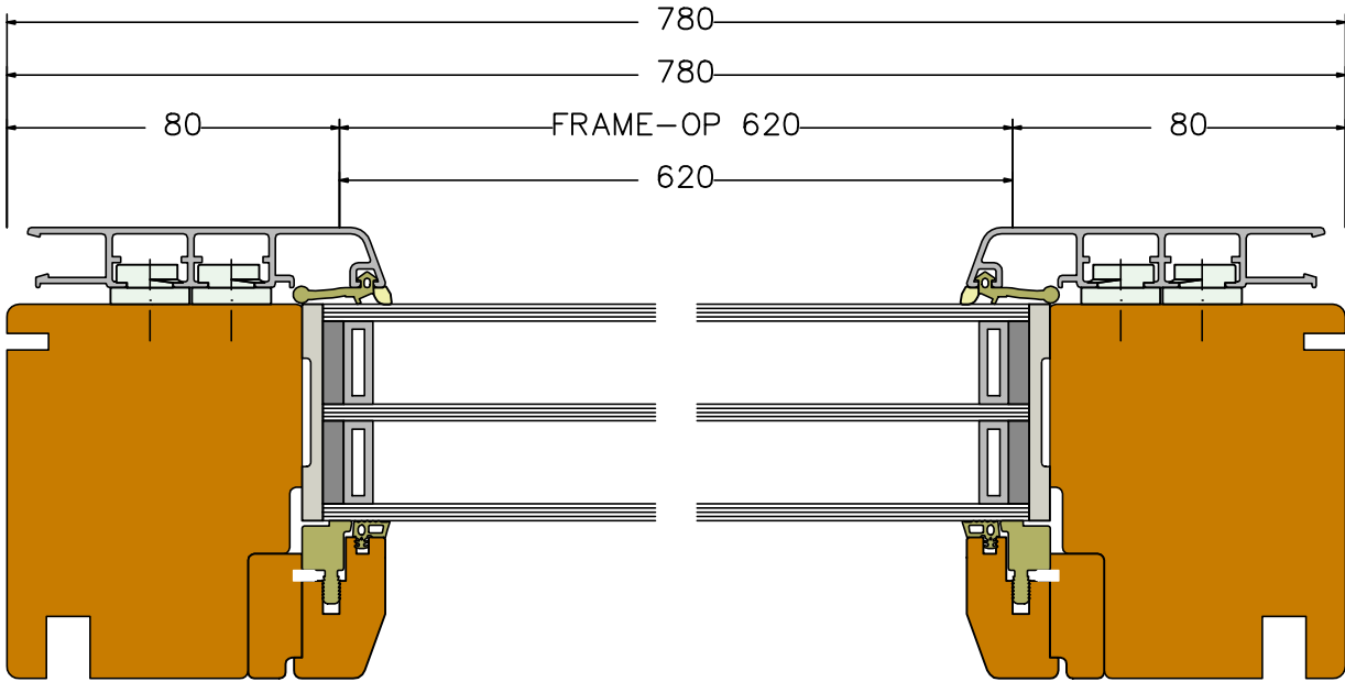
Section H1 (scale 1:2)
