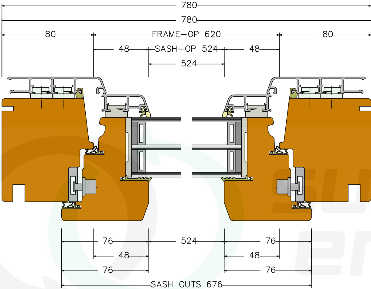
Section H2 (scale 1:2)
